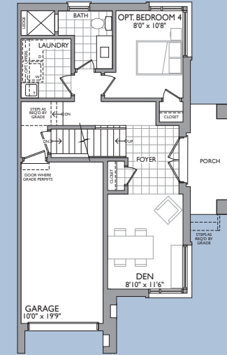
OPT. FIRST FLOOR LOT: 52
