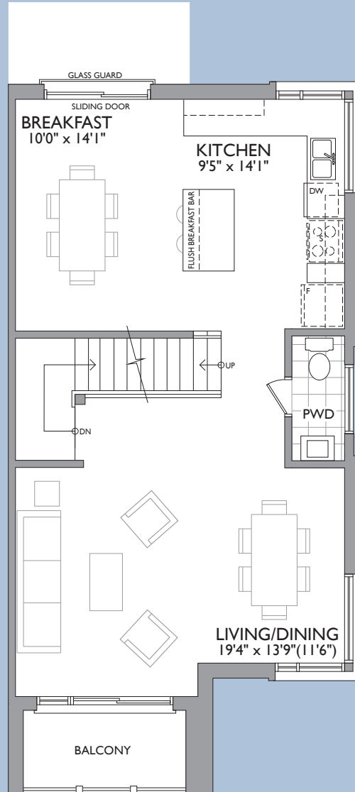
SECOND FLOOR LOTS: 52, 53, 67
